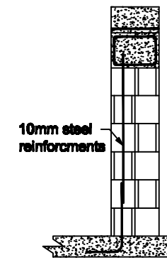
Section C-C
