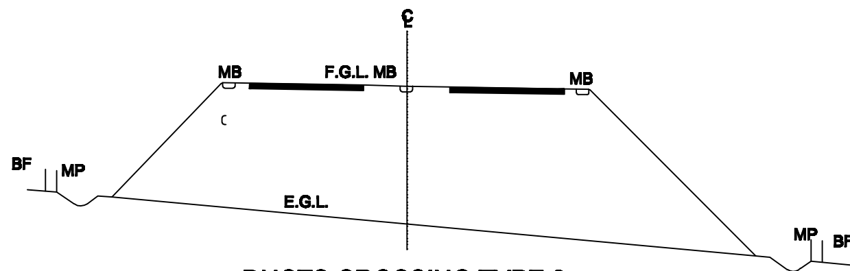
DUCTS CROSSING TYPE 2. (FILL AREAS) N.T.S.
