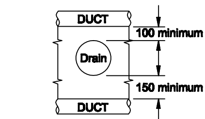
MINIMUM CLEARANCE BETWEEN DUCT AND DRAIN
