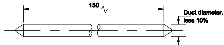
DETAIL OF MANDREL
