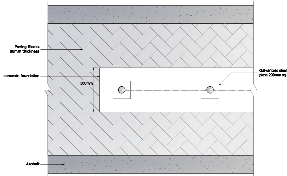
Detailed Plan
