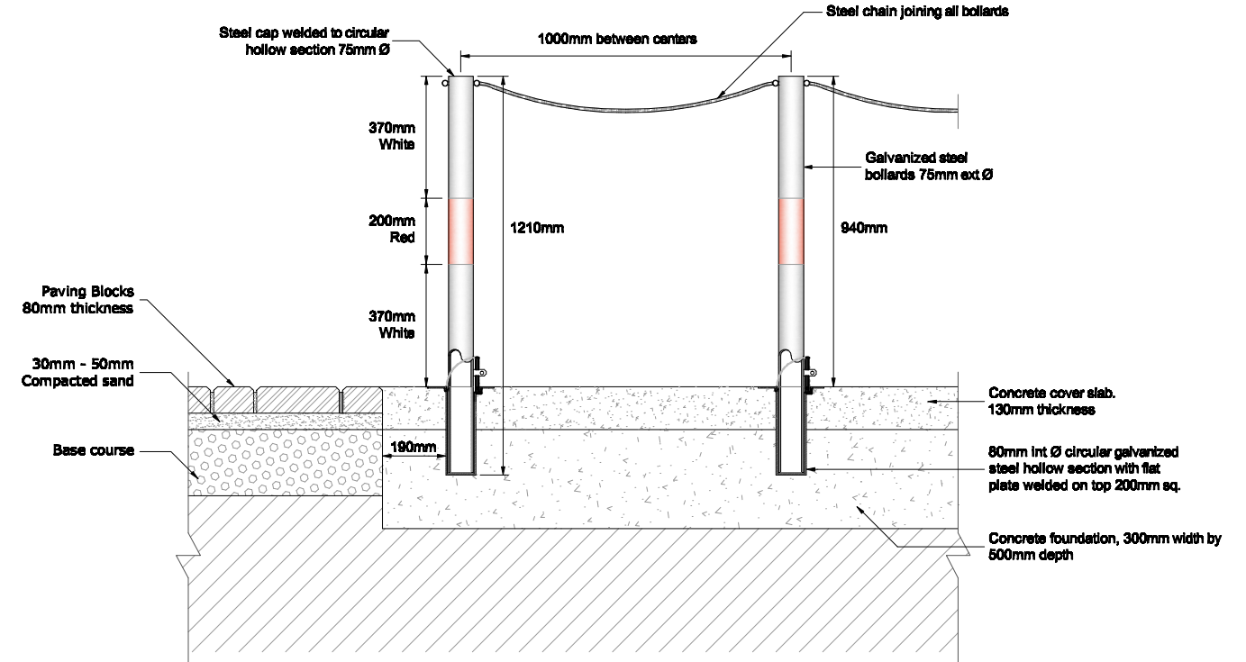
Sectional Elevation
