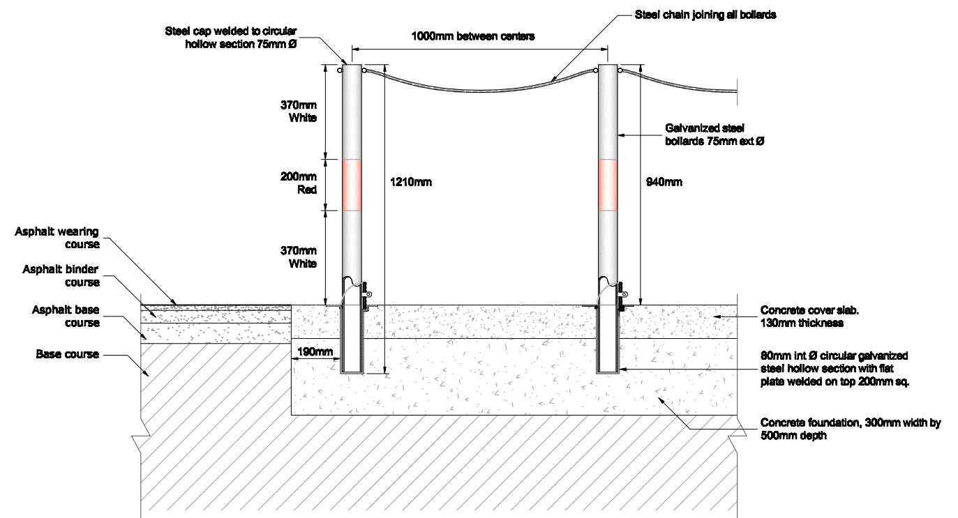
Sectional Elevation
