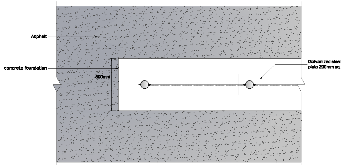
Detailed Plan
