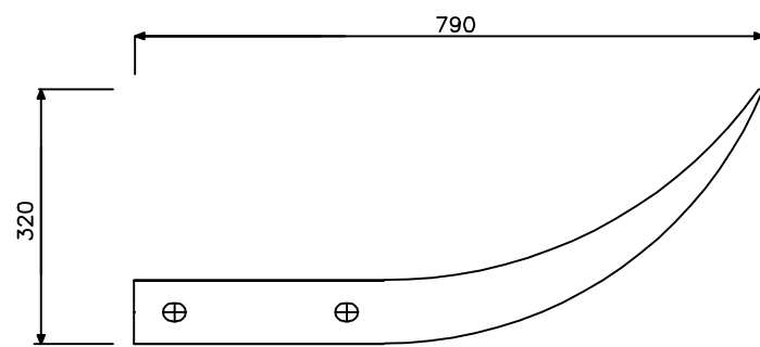
Scale 1 : 10 Detail of fishplate
