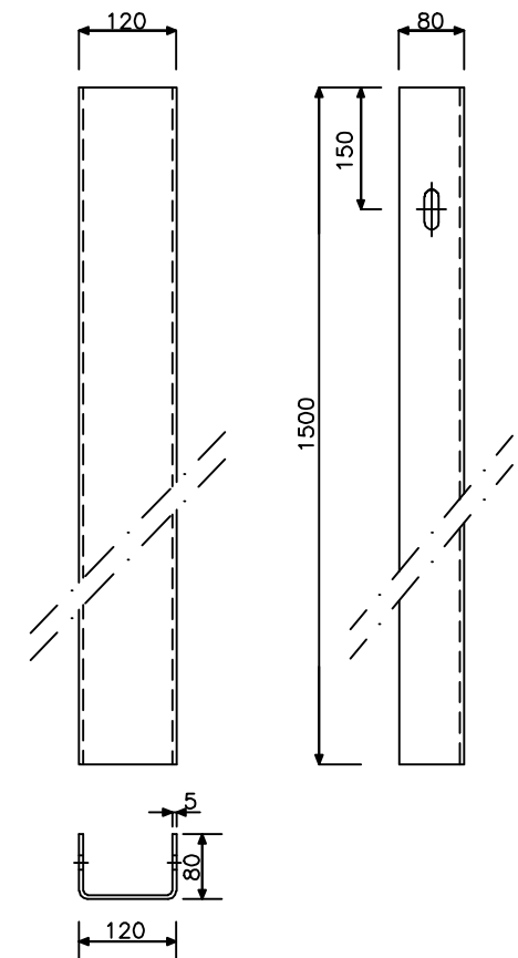
Scale 1 : 10 Detail of post
