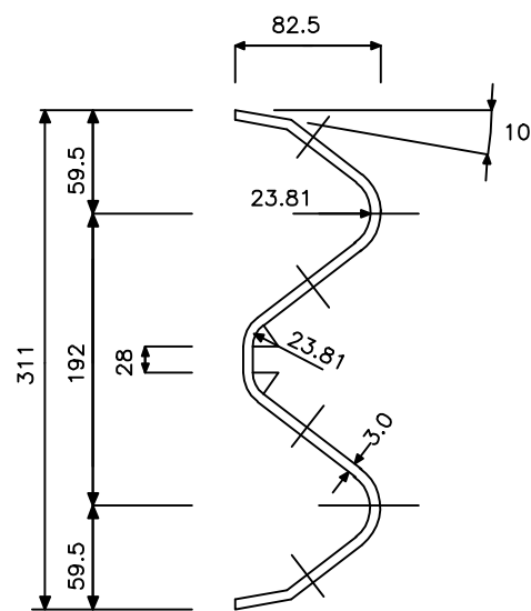
Scale 1 : 5 Detail of fender
