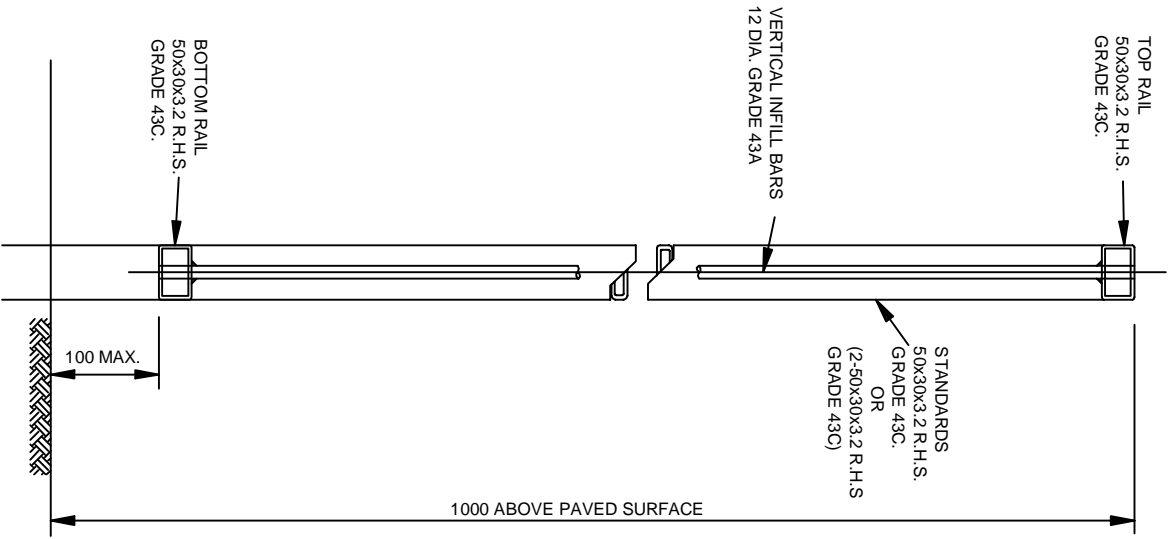
TYPICAL SECTION THROUGH GUARDRAIL
