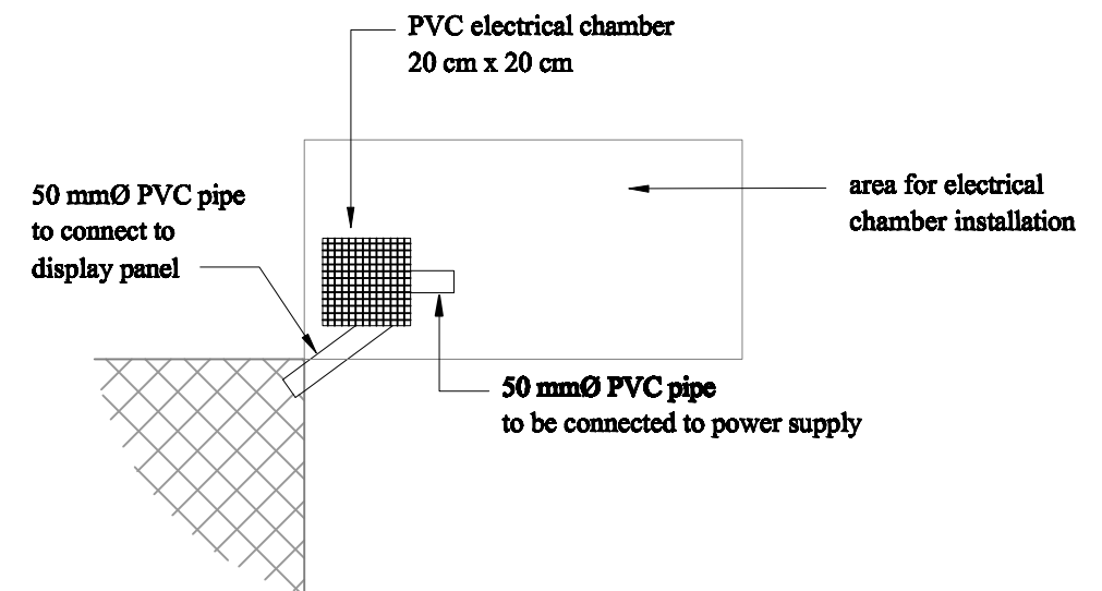
Detail C
