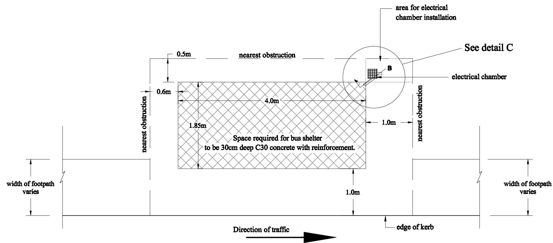
Plan for bus shelter foundation
