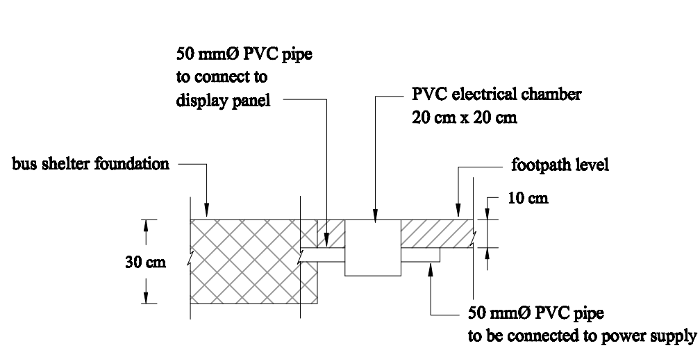
Part section through electrical inspection box - section B
