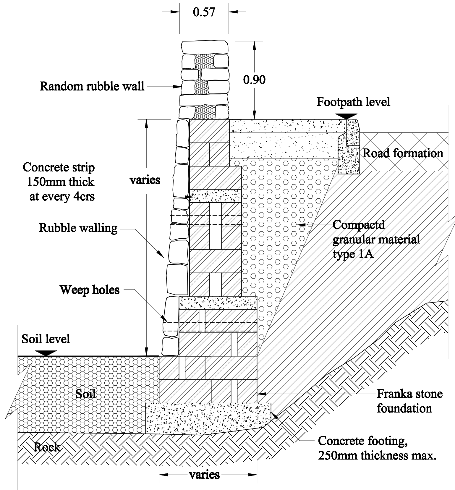
Type K Boundary wall retaining road
