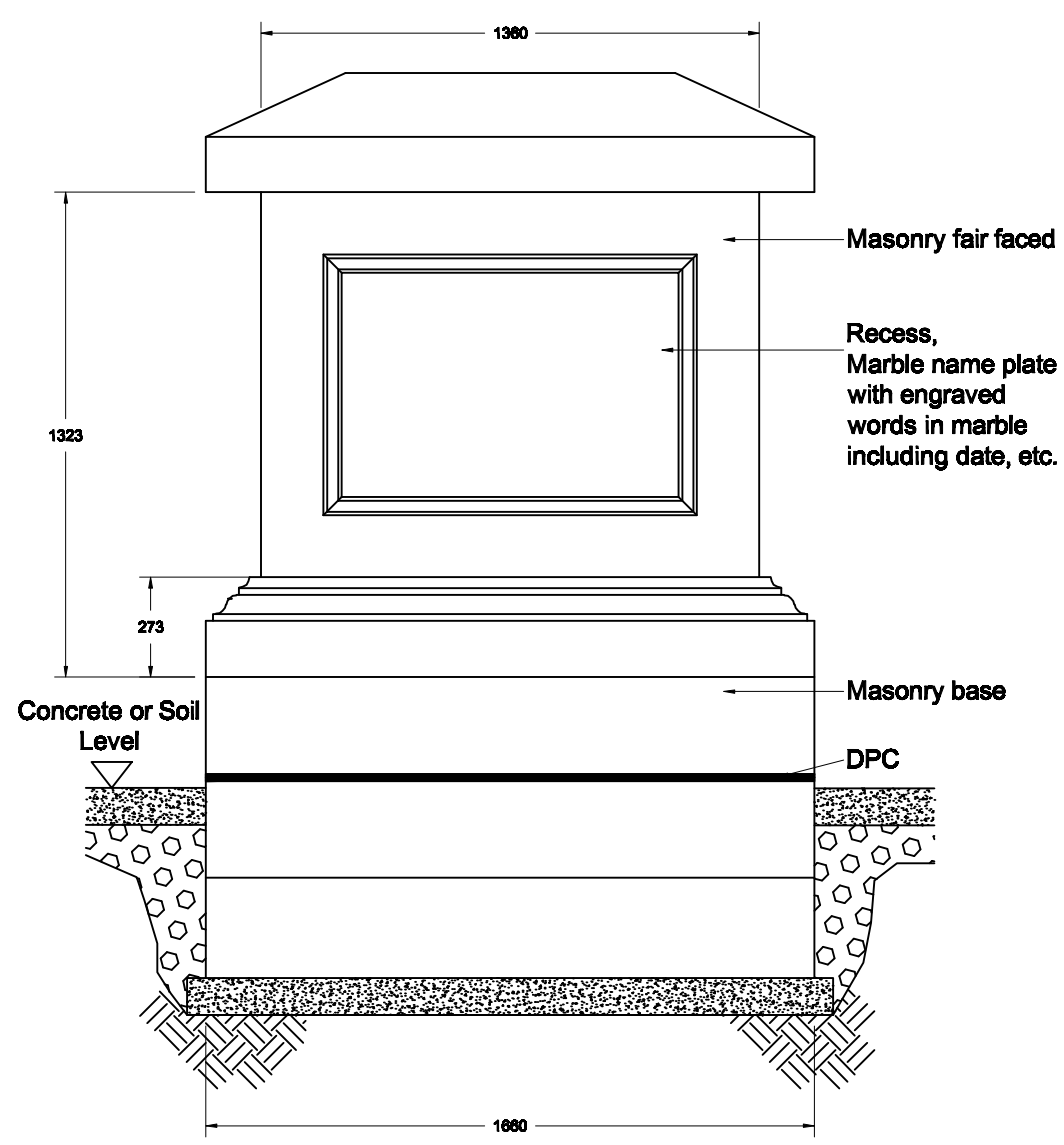
Front Elevation
