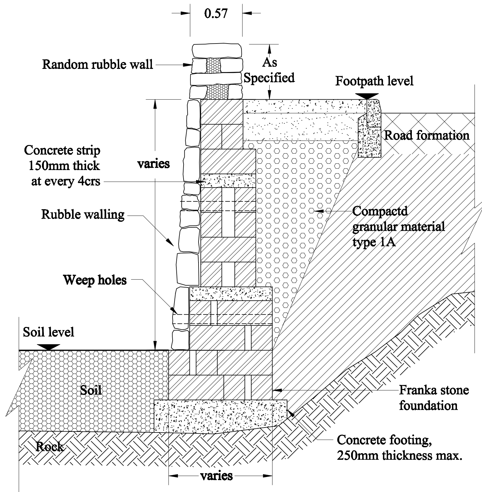
Type F Boundary wall retaining road
