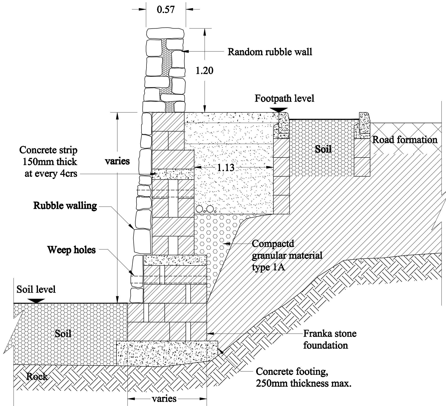
Type E Boundary wall retaining road
