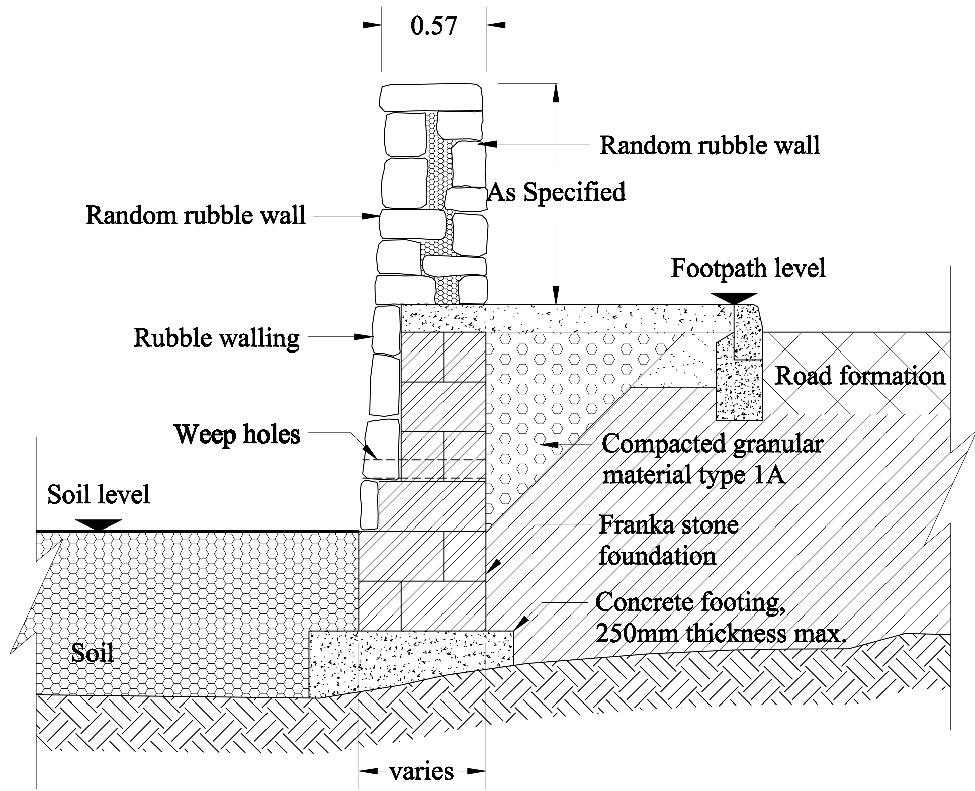
Type C Boundary wall retaining road
