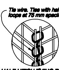
HALF HITCH TYING DETAIL (Welded wire mesh)
