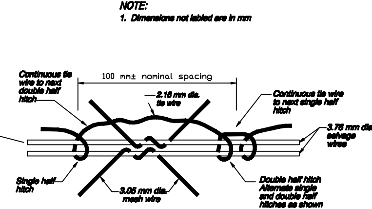
HALF HITCH TYING DETAIL (Twisted wire mesh)
