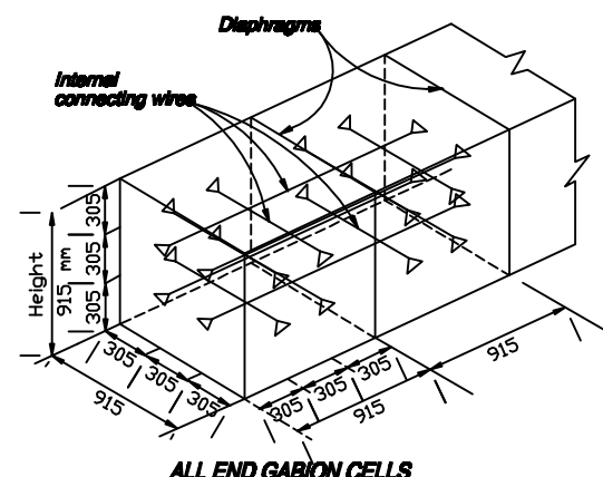
TYPICAL INTERNAL CONNECTING WIRES
