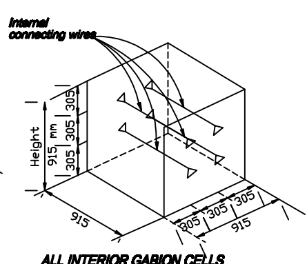
TYPICAL INTERNAL CONNECTING WIRES
