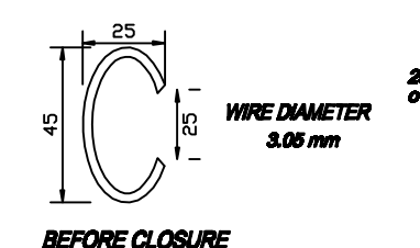
INTERLOCKING WIRE FASTNER OVERLAPPING RING WIRE FASTNER (Not allowed for basket to basket connection) ALTERNATE TYING FASTNERS
