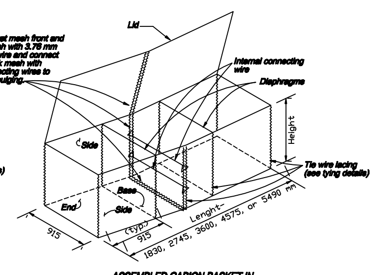
ASSEMBLED GABION BASKET IN WALL GRADE TRANSITION AREAS
