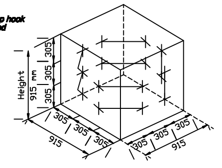
ALL GABION CELLS OPTIONAL INTERNAL CONNECTING WIRES WELDED WIRE GABION BASKET
