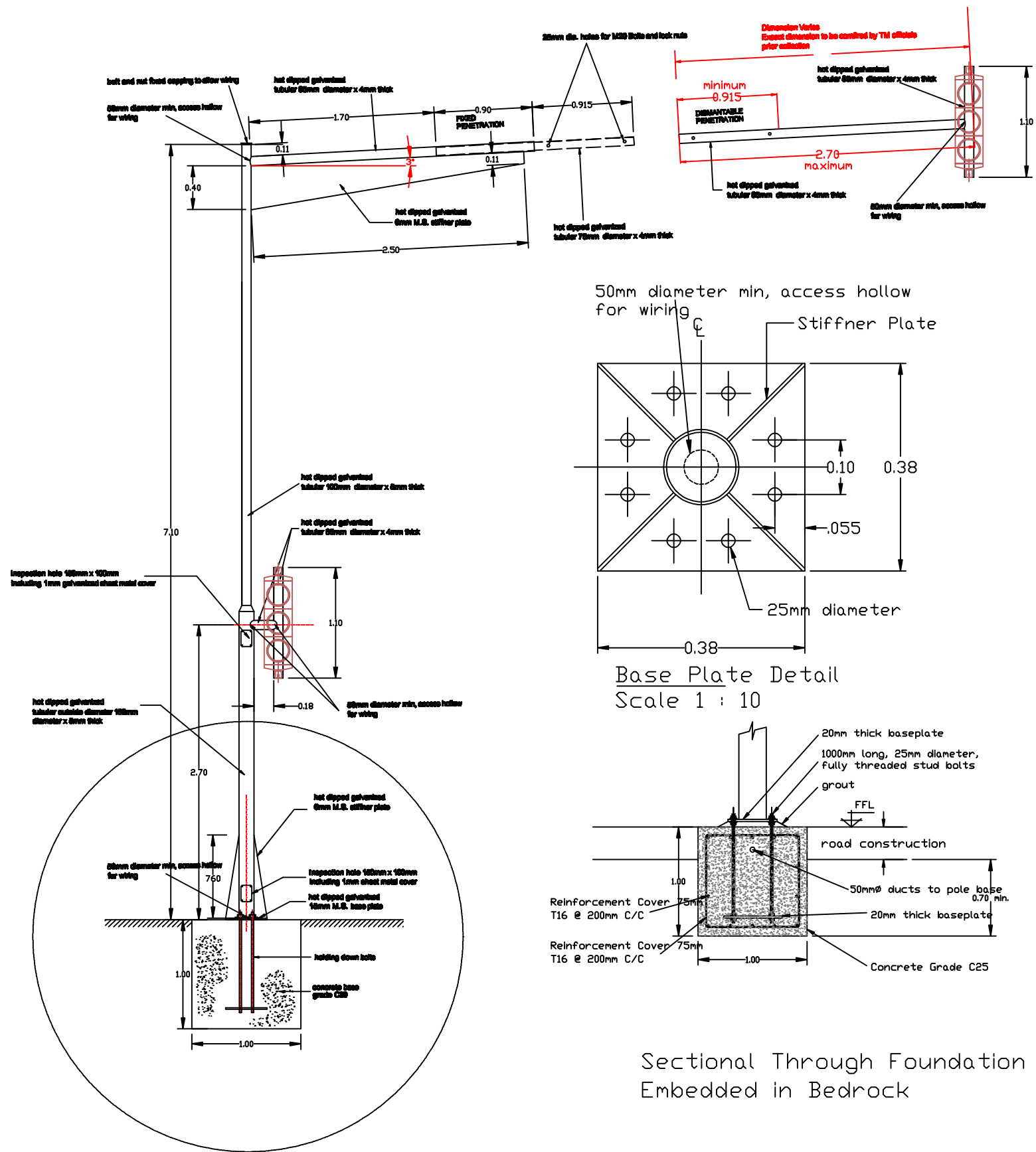
Pelican Lights With Overhead Scale 1 : 50
