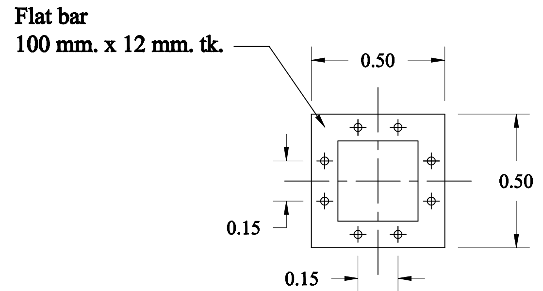
Anchor Plate
