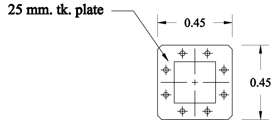
Base Plate
