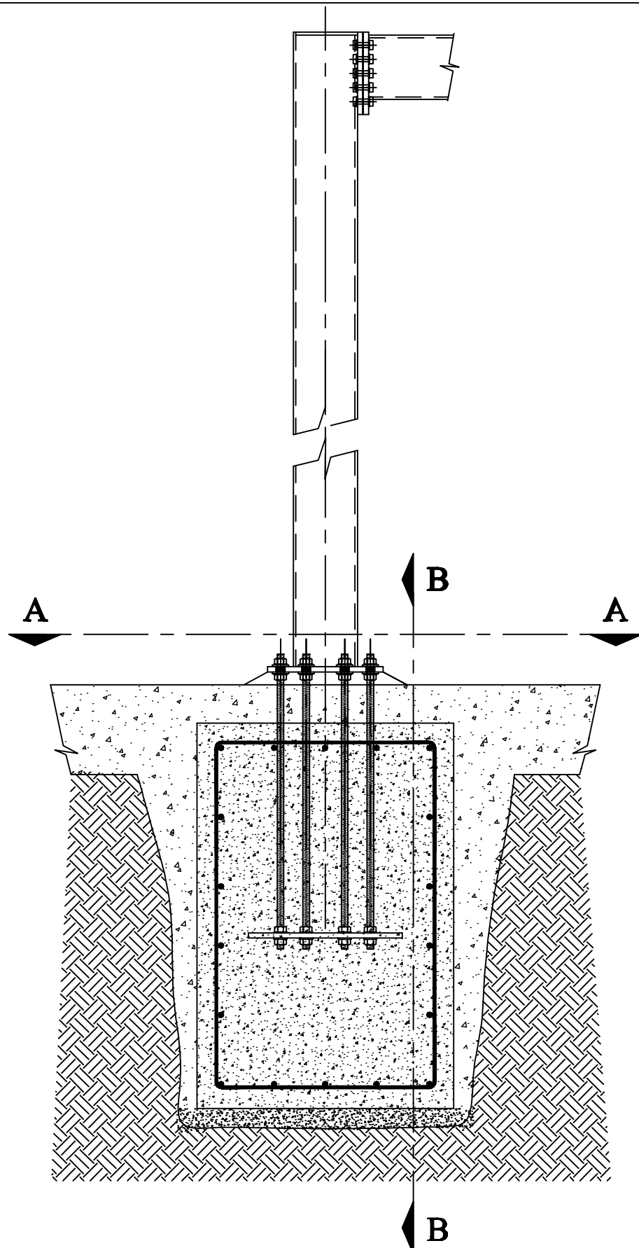
Sectional Elevation
