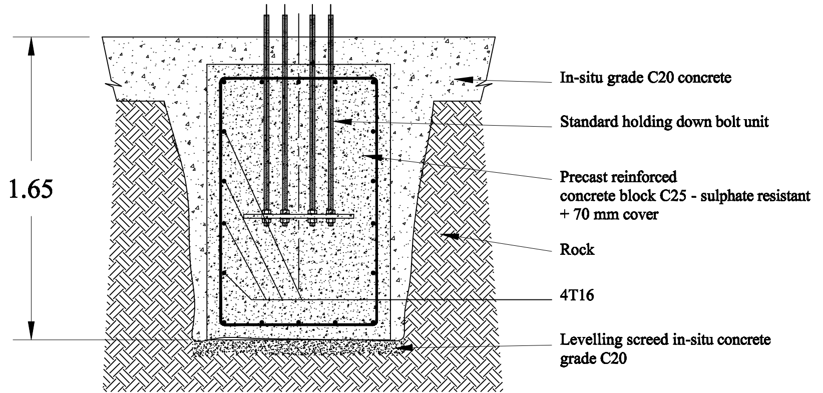
Section B-B
