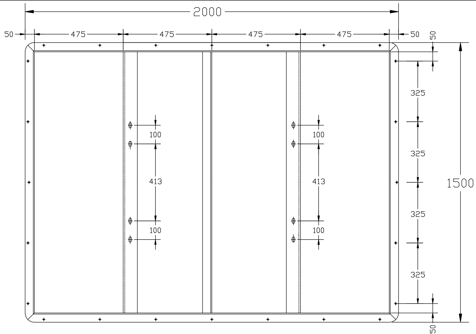
Inner Frame of Signboard (2000mm x 1500mm)
