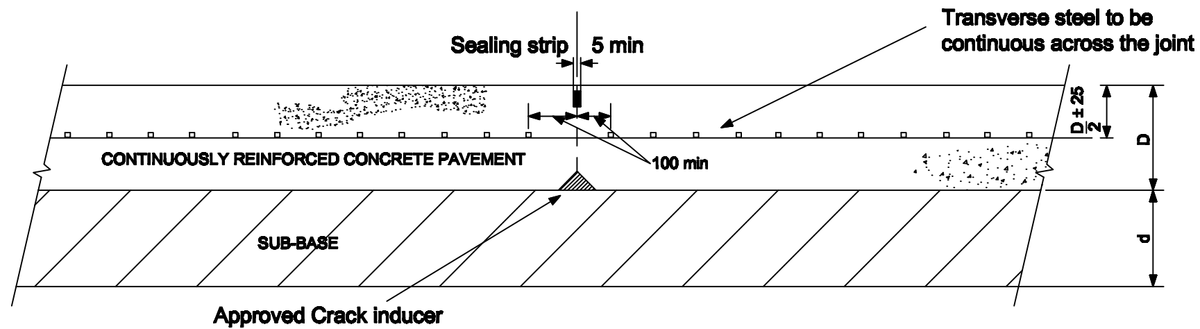
FORMED LONGITUDINAL JOINT FOR CRCP OR CRCR (constructed in more than one lane width in one operation)
