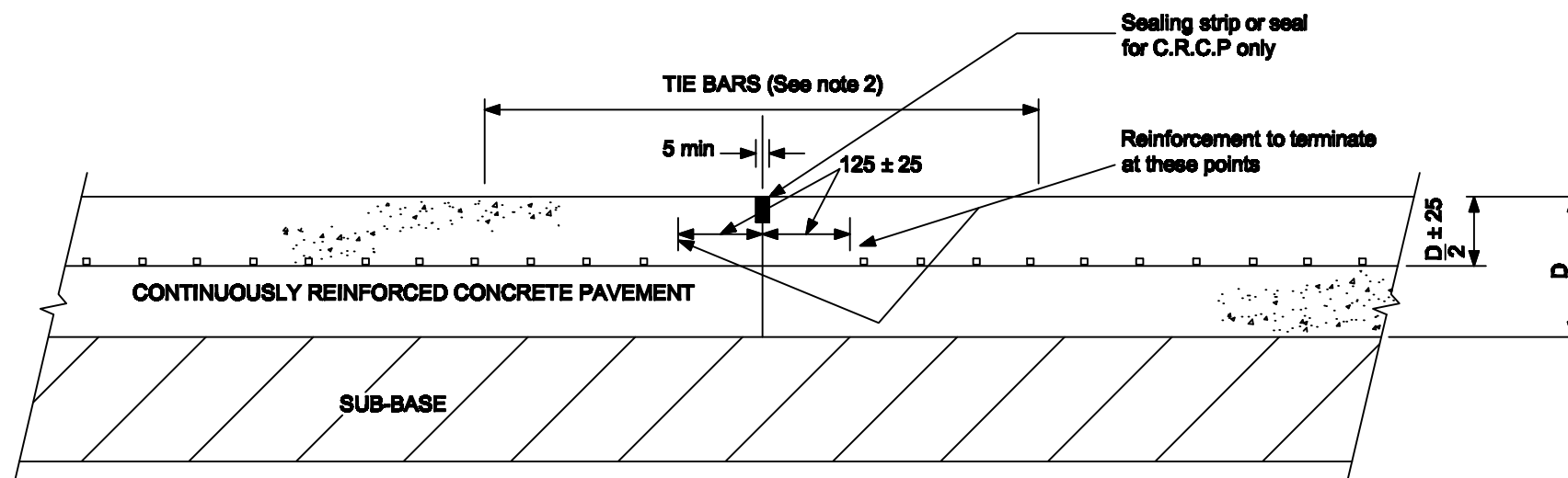
CRCP or CRCR BUTT TYPE CONSTRUCTION JOINT (between separately constructed slabs)
