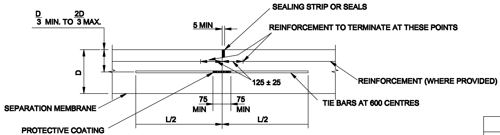
TYPE 3 SAWN LONGITUDINAL JOINT FOR UNREINFORCED OR JOINTED REINFORCED SLABS (MORE THAN ONE LANE WIDTH CONSTRUCTED IN ONE OPERATION)
